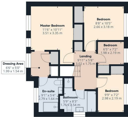
Floor 1
