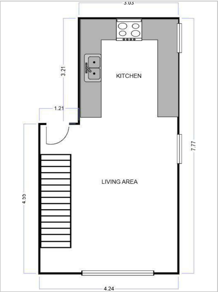
Floor Plan
