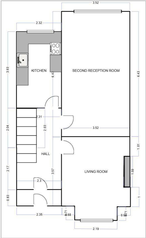
Floor Plan
