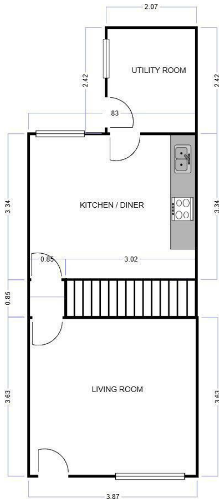
Floor Plan
