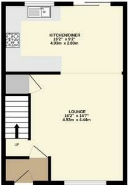
GROUND FLOOR 384 sq.ft. (35.7 sq.m.) approx.
