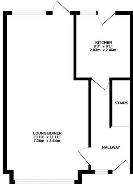
GROUND FLOOR 414 sq.ft. (38.5 sq.m.) approx.
