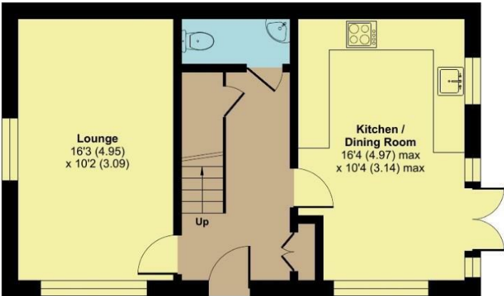
GROUND FLOOR APPROX FLOOR AREA 42.7 SQ M (460 SQ FT)
