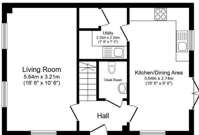
Ground Floor Floor area 47.1 sq.m. (507 sq.ft.)
