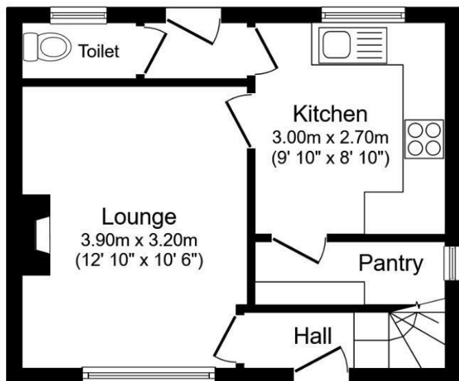
Ground Floor Floor area 26.7 sq.m. (287 sq.ft.)
