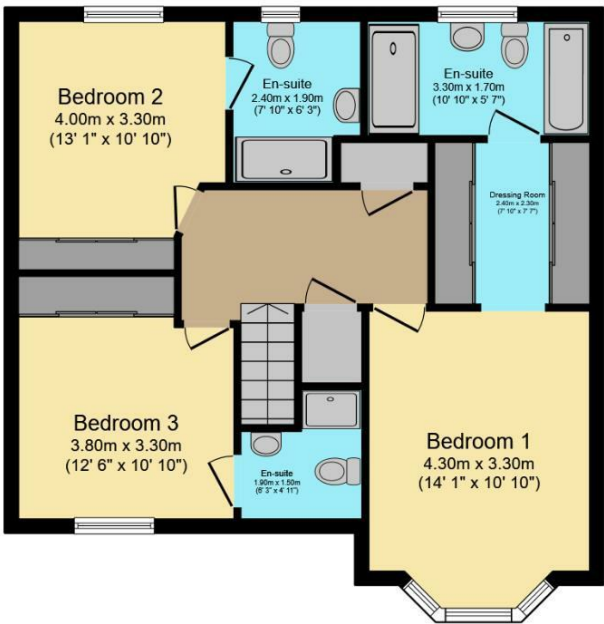
First Floor Floor area 66.1 sq.m. (712 sq.ft.)
