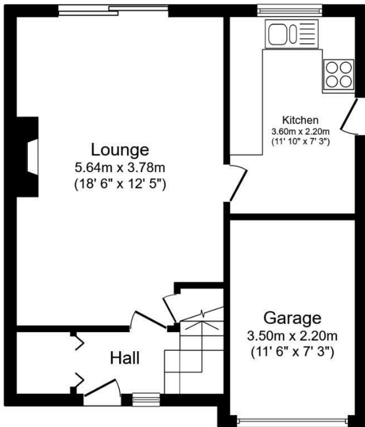
Ground Floor Floor area 43.4 sq.m. (467 sq.ft.)
