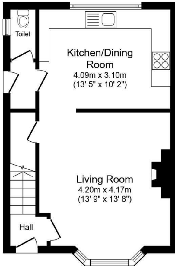
Ground Floor Floor area 37.7 sq.m. (405 sq.ft.)
