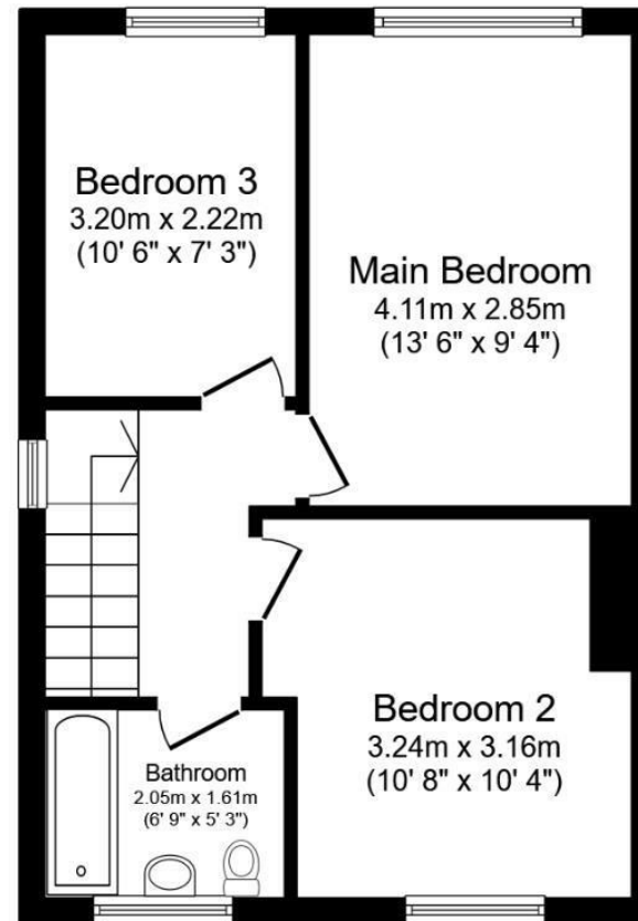
First Floor Floor area 36.9 sq.m. (398 sq.ft.)
