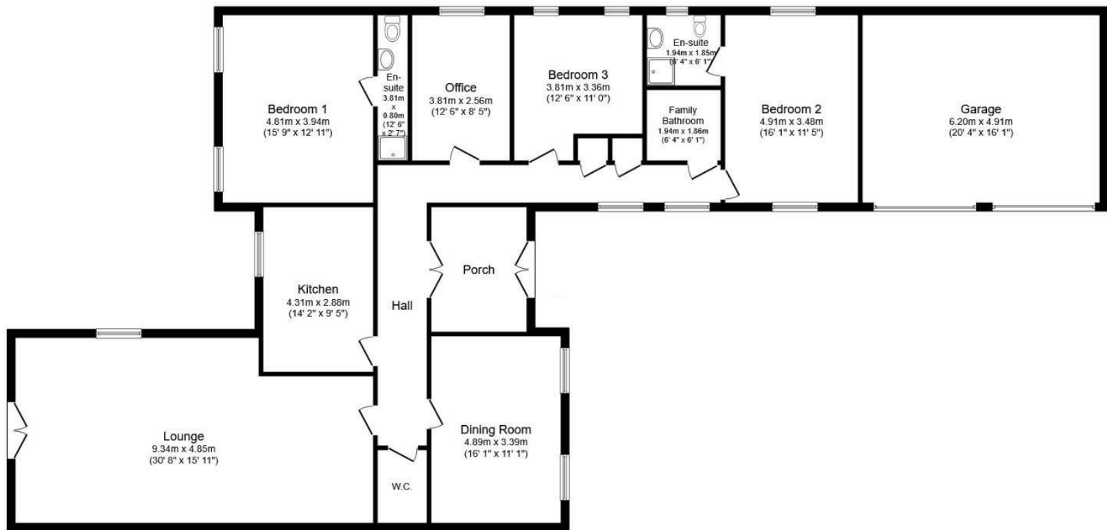
Floor Plan Floor area 205.5 sq.m. (2,212 sq.ft.)
