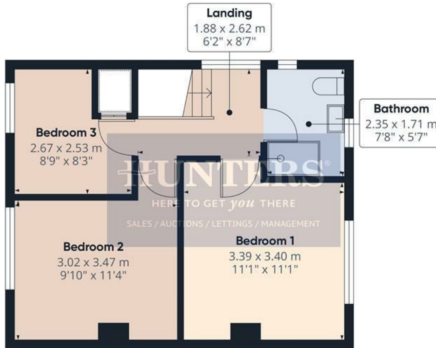
Floor 1
