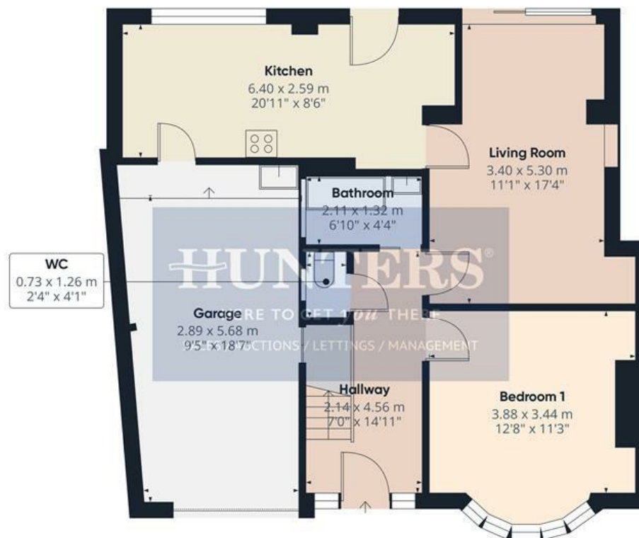
Floor 0
