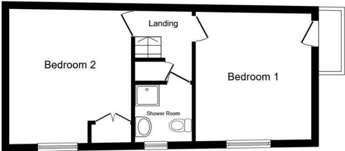
First Floor
