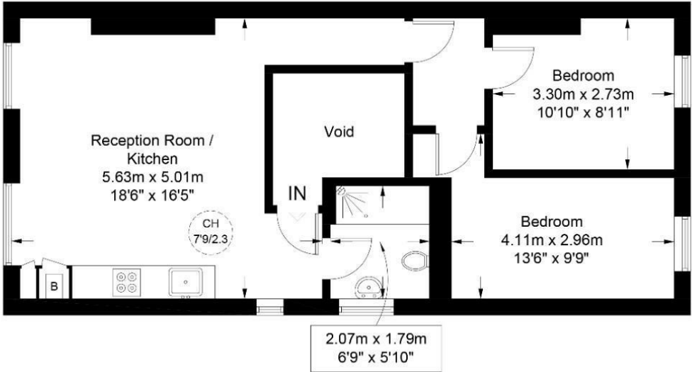
Third Floor
