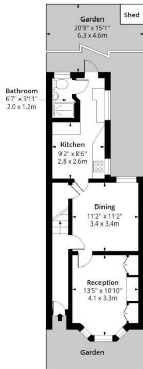
Ground Floor Floor Area 473 Sq Ft - 43.94 Sq M
