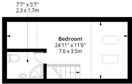
Second Floor Floor Area 295 Sq Ft - 27.41 Sq M
