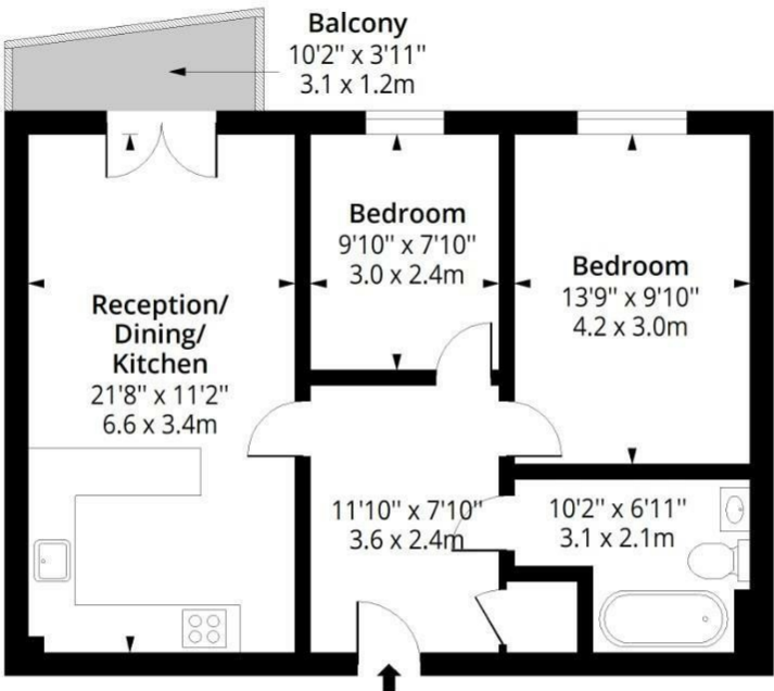
Second Floor Floor Area 654 Sq Ft - 60.76 Sq M
