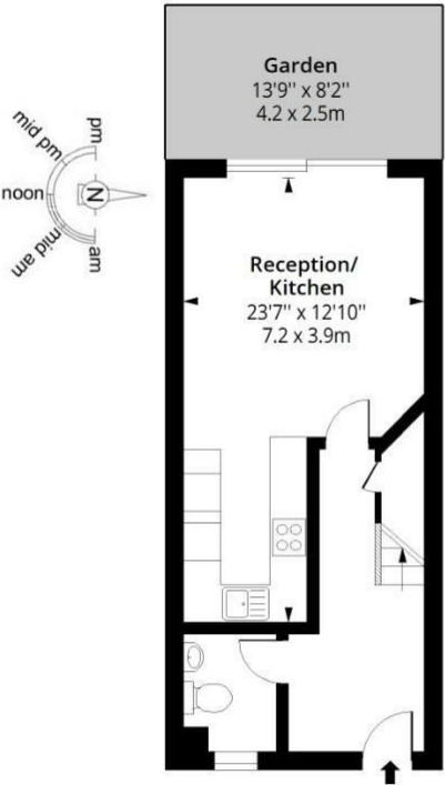
Ground Floor Floor Area 390 Sq Ft - 36.23 Sq M
