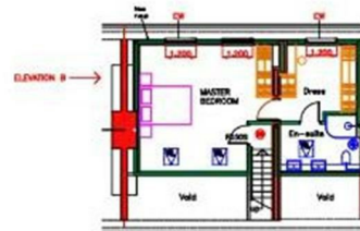
LOFT SPACE PLAN as proposed
