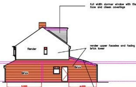
END ELEVATION as proposed
