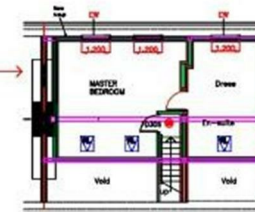
LOFT SPACE STUCTURE PLAN
