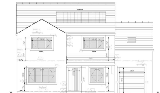
SOUTH ELEVATION
