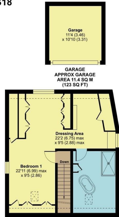
SECOND FLOOR APPROX FLOOR AREA 46.3 SQ M (499 SQ FT)
