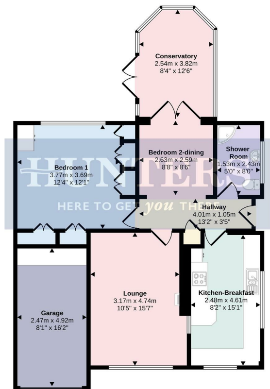
Floorplan
