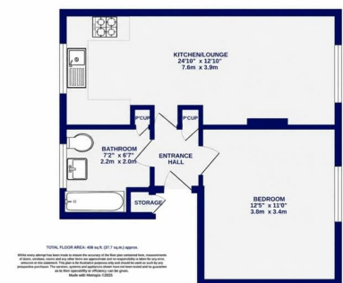
FIRST FLOOR 406 sq.ft. (37.7 sq.m.) approx.
