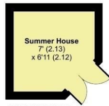
OUTBUILDING 2 APPROX FLOOR AREA 4.1 SQ M (45 SQ FT)
