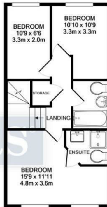
2ND FLOOR APPROX. FLOOR AREA 424 SQ.FT. (39.4 SQ.M.)
