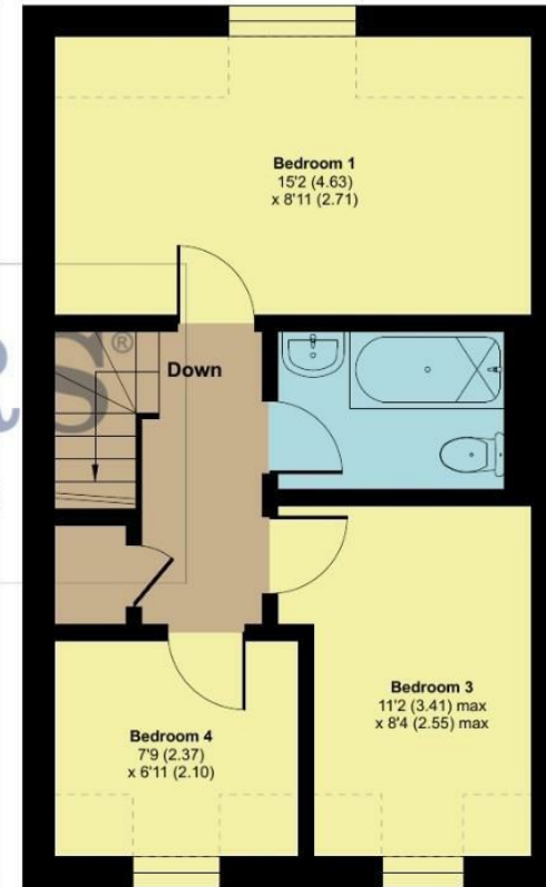
SECOND FLOOR APPROX FLOOR AREA 32.9 SQ M (355 SQ FT)
