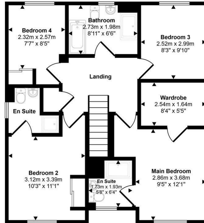
First Floor Approx 68 sq m / 730 sq ft
