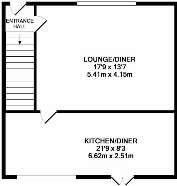
GROUND FLOOR APPROX. FLOOR AREA 475 SQ.FT. (44.1 SQ.M.)
